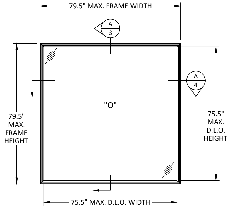
ELEVATION UNIT 3
