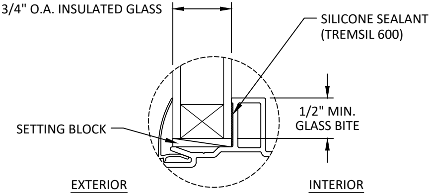
GLAZING DETAIL
