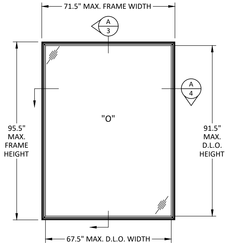
ELEVATION UNIT 1
